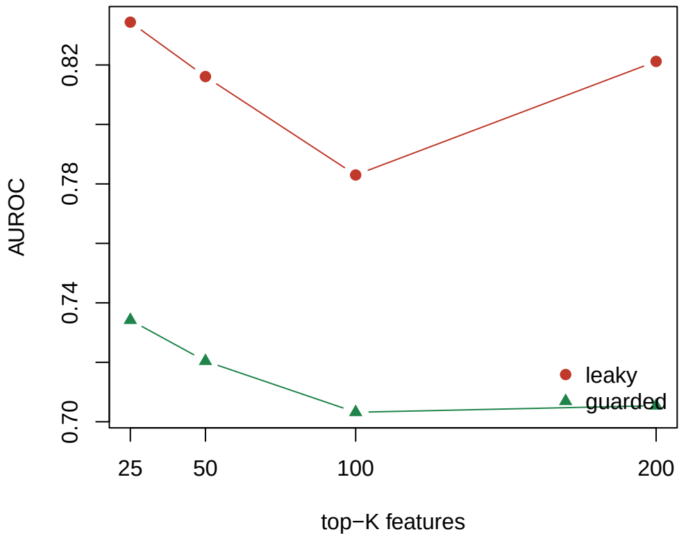
Leaky vs guarded AUROC by K
