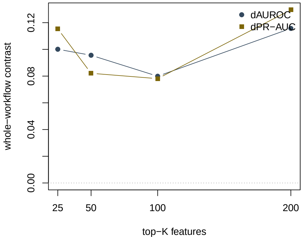
Naive – guarded contrast by K
