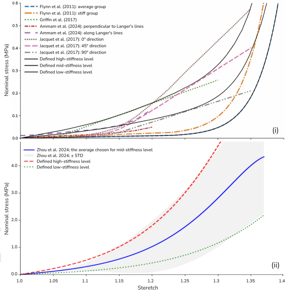
Fig 4. Literature review of experimental data on the material parameters for the Forearm skin (i) and the Thigh skin (ii) represented as the stress-stretch response to a uniaxial tensile test.
