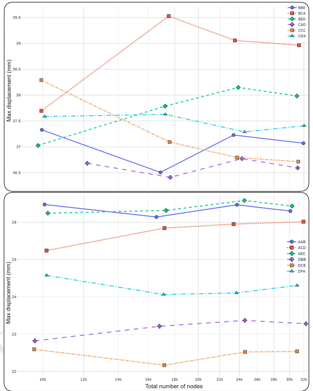
S2 Fig. Mesh convergence analysis—Maximum displacement. Maximum nodal displacement of the neotongue at the final post-remodeling equilibrium (mm) versus total mesh nodes for 12 representative parameter combinations (same [Case][Donor/Stiffness][Overbulking] codes as in S1 Fig). Two panels are shown for better readability; horizontal axis is shared.
