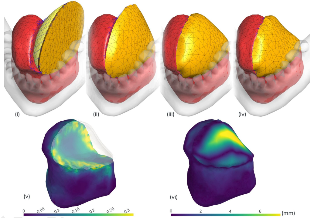
Fig 3. Surgical simulation pipeline: reconstruction to long-term remodeling. (i) Initial simulation setup, (ii) The suture model brings the flaps proximal to the resected tongue model and simulates suturing. (iii) After the 5-minute idling for stresses to relax with the viscoelastic model present, this is "Day 0" immediately after reconstruction. (iv) shows the tongue model after one-year of post-surgery atrophy modeling. At the very end, the effective strain (v) and Hausdorff distance (vi) are calculated and used for the statistical analysis.
