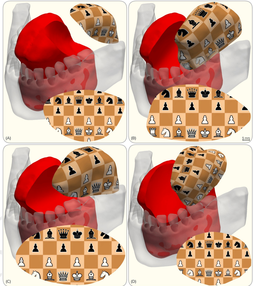
Fig 1. Patient-Specific Tongue Model, Resection Scenarios, and Flap Designs. Overview of the four simulated tongue cancer cases along with their biomechanically-optimized flap designs. The texture mapping is generated with hiFEM and maps each point in the resection model to its corresponding point in the planar flap design.
