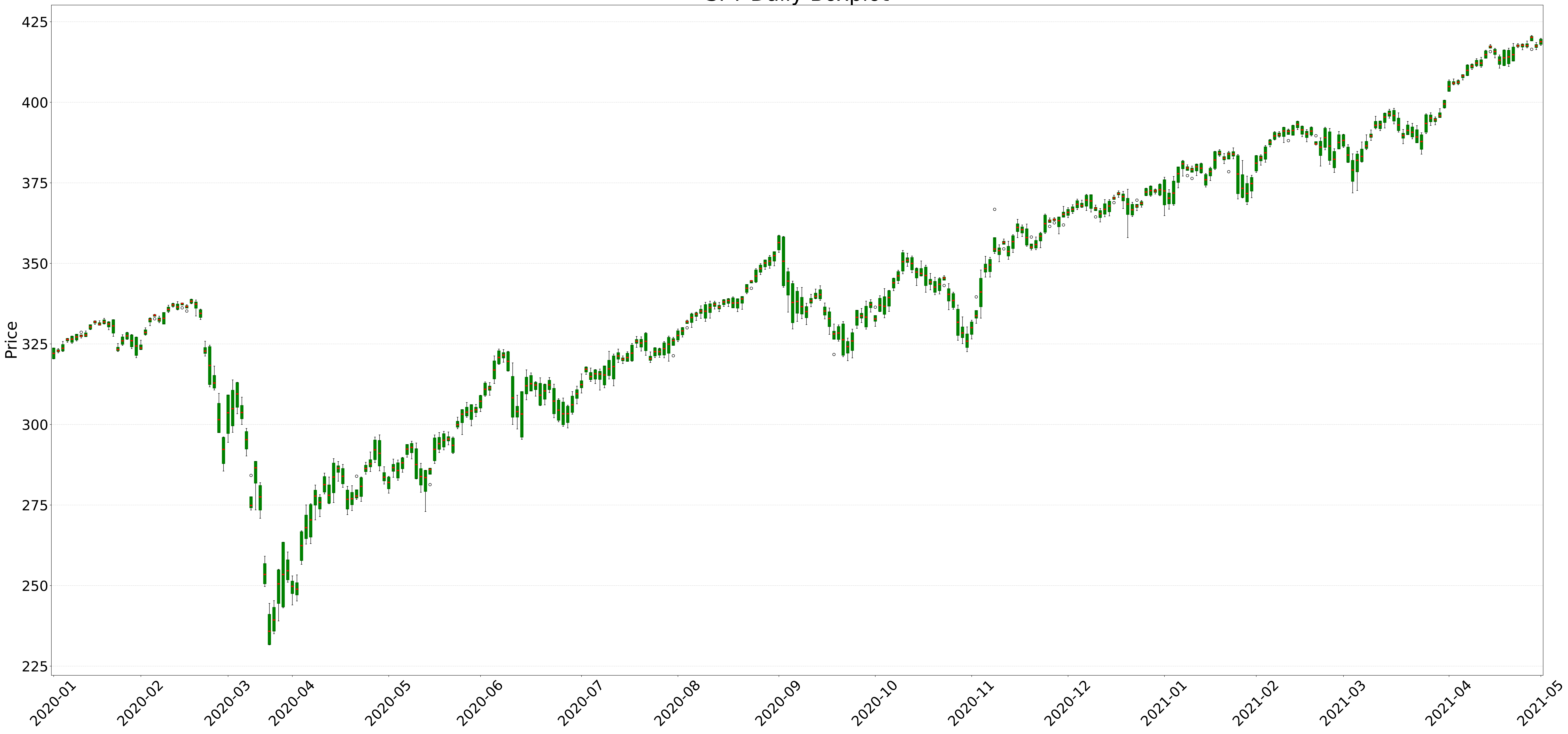
SPY Daily Boxplot
