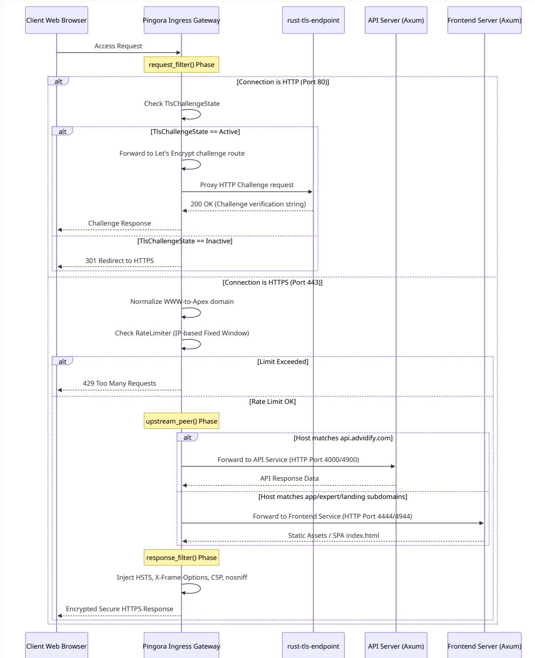
Figure 2: Request Lifecycle & Routing Control Flow
