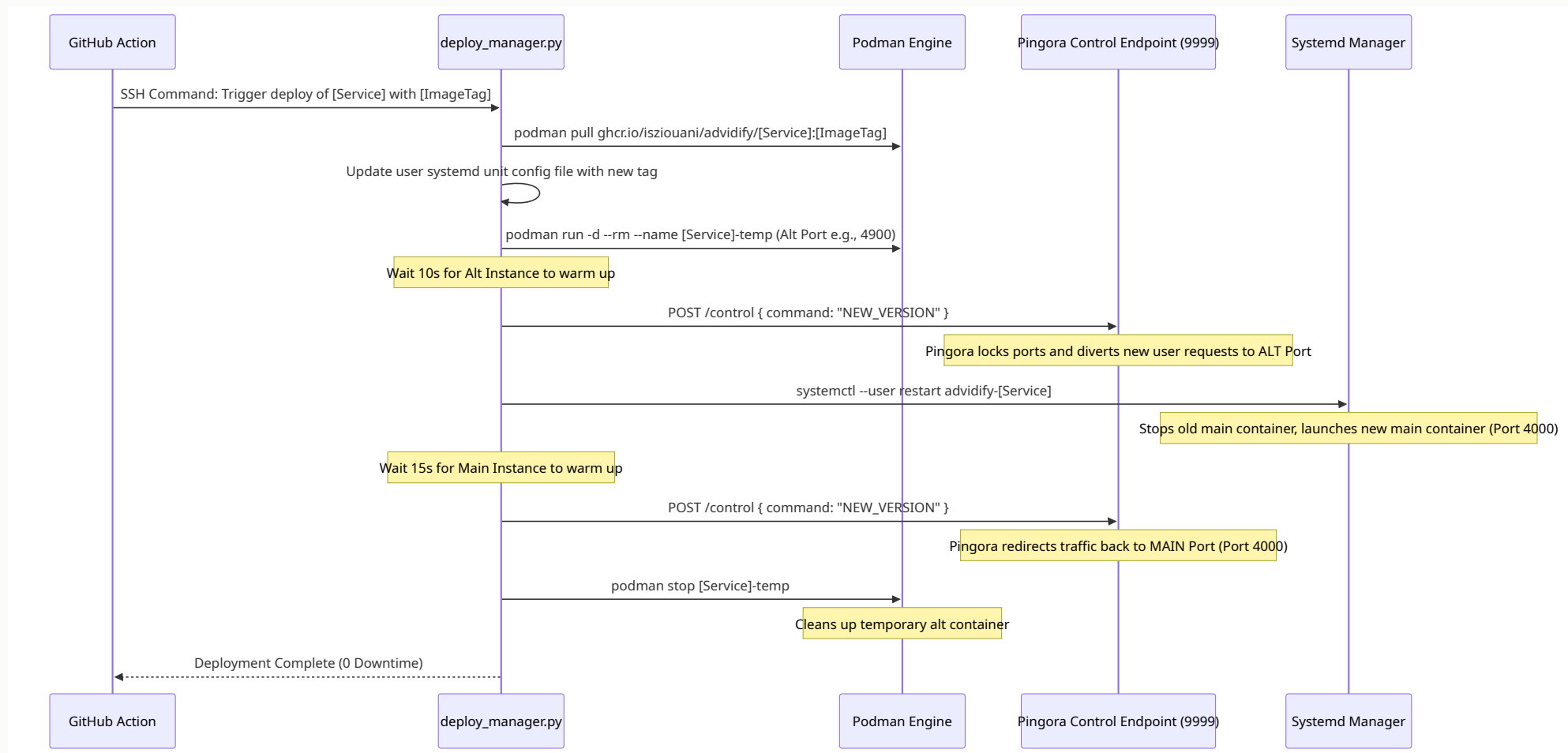
Figure 3: DevOps Pipeline: Zero-Downtime Blue-Green Deployment
