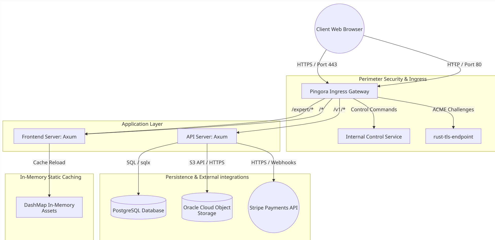
Figure 1: Overarching System Architecture
