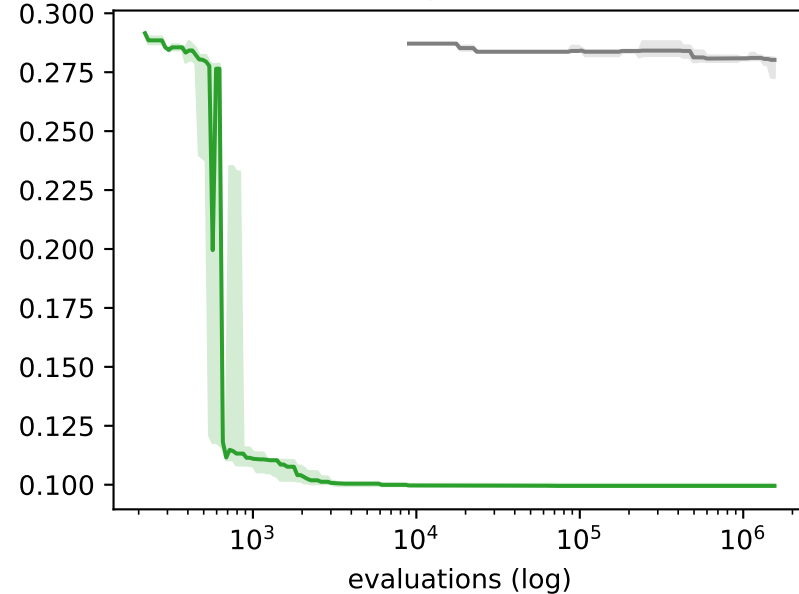
arOrch @ 135 nodes
