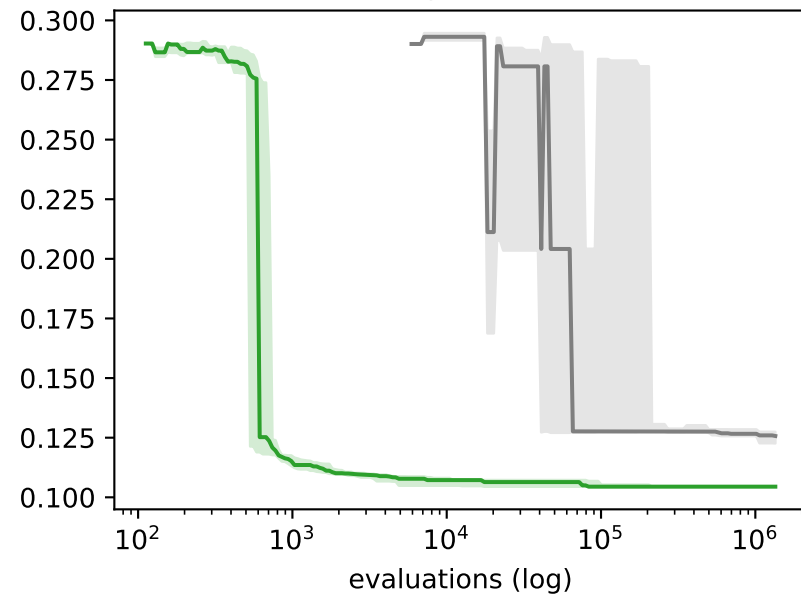
arOrch @ 220 nodes
