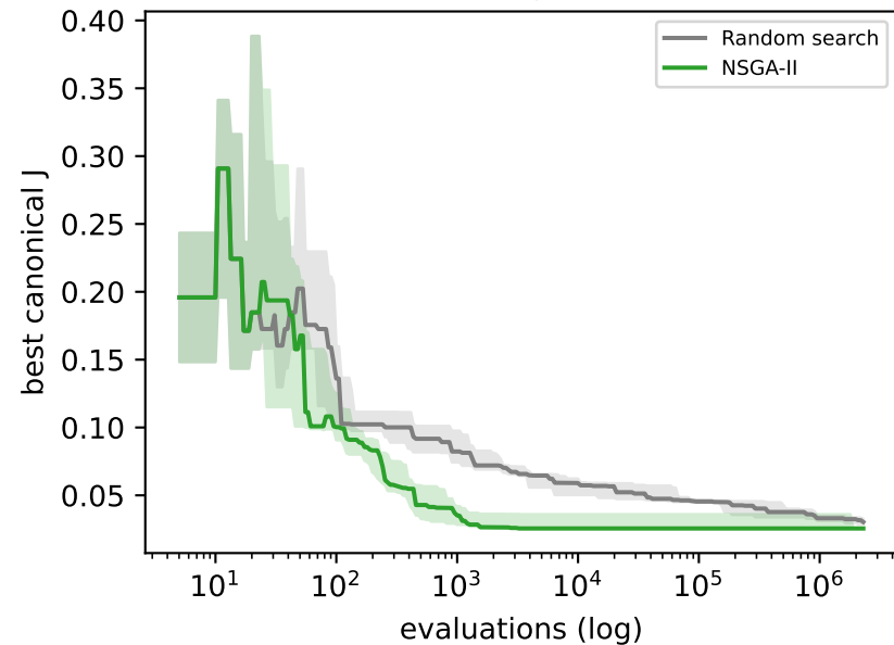
mediaOrch @ 50 nodes
