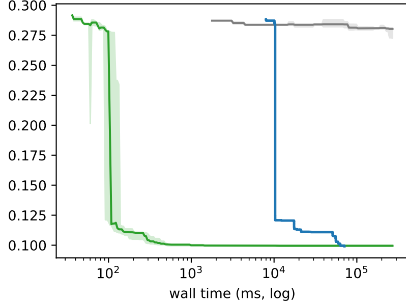
arOrch @ 135 nodes
