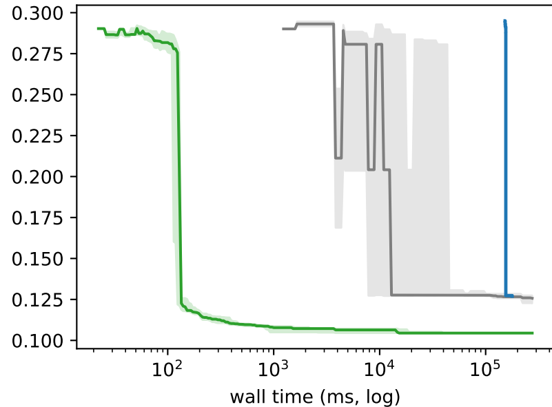
arOrch @ 220 nodes
