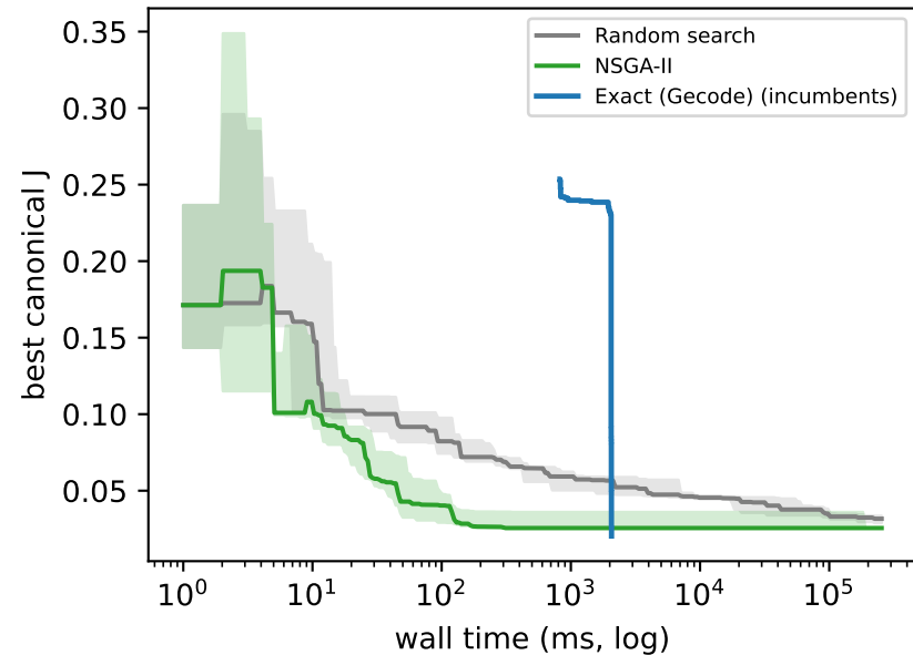
mediaOrch @ 50 nodes
