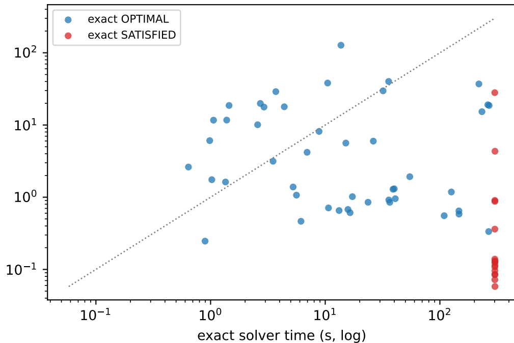
NSGA-II median time over 10 seeds to within 1% of reference (s, log)
