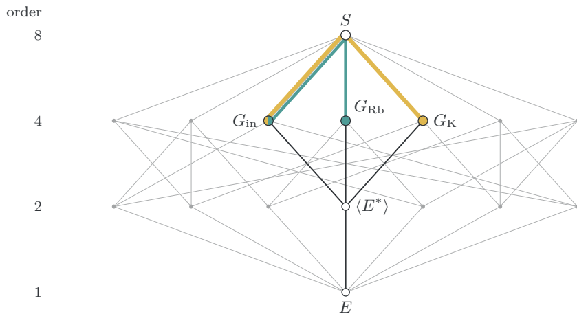
KRb + KRb G_{\text{in}} = \langle (12)(34), E^* \rangle
