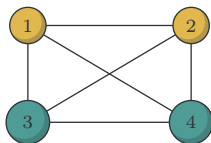
\text{K}_2\text{Rb}_2 S = \langle (12), (34), E^* \rangle
