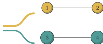
\text{K}_2 + \text{Rb}_2 G_{\text{K}} = \langle (12), E^* \rangle, G_{\text{Rb}} = \langle (34), E^* \rangle
