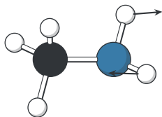
e_-(q) , the amino twist
