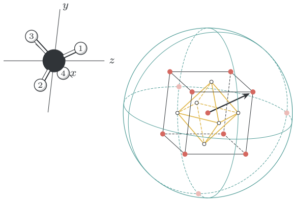
The orientation space SO(3) as a ball, direction the axis and distance the angle: the twelve rotations of T , the cell \mathcal{U} at q = 0 in gold, and the lift r \rightarrow r\mathbf{R}_g of the third-turn loop.
