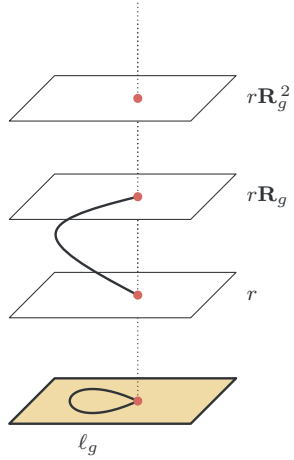
The covering SO(3) \rightarrow SO(3)/T , as in Figure 11: three of the twelve sheets, one per rotation in T ; the loop \ell_g in the base, and its lift from sheet r to r\mathbf{R}_g . A sees 1, {}^1\text{E} sees \omega , {}^2\text{E} sees \omega^2 , and T cycles x, y, z .
