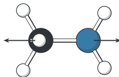
\mathbf{e}_+(a) , the C-N stretch
