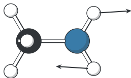
e_-(q) , the amino twist
