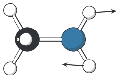
e_-(q) , the amino twist
