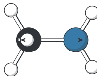
e_+(q) , the C-N stretch
