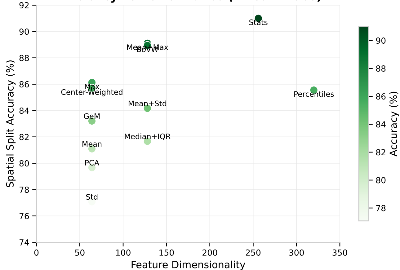
Efficiency vs Performance (Linear Probe)
