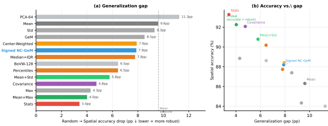
Fig. 3. Distributional pooling is more accurate and more robust under spatial shift. (a) Accuracy drop when moving from a random to a geographically disjoint split, averaged across three GFMs—shorter bars are better. Mean pooling drops 9.6pp; stats drops only 3.4pp, a 65% reduction. (b) Spatial accuracy vs. generalization gap per method. Methods in the upper-left are both accurate and robust; distributional methods cluster there while mean pooling sits lower-right.
