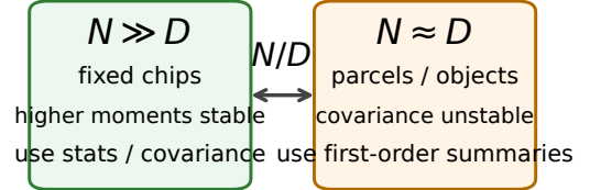
same embedding product, different region size \rightarrow different pooling rule
