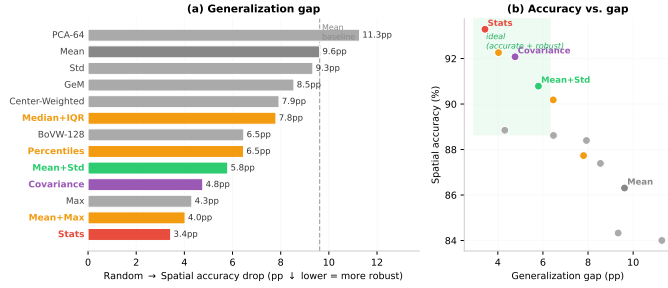
Fig. 3. Distributional pooling is more accurate and more robust under spatial shift. (a) Accuracy drop when moving from a random to a geographically disjoint split, averaged across three GFM—shorter bars are better. Mean pooling drops 9.6pp; stats drops only 3.4pp, a 65% reduction. (b) Spatial accuracy vs. generalization gap per method. Methods in the upper-left are both accurate and robust; distributional methods cluster there while mean pooling sits lower-right.
