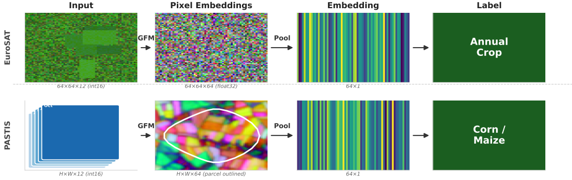
Fig. 1. Embedding pipeline for EuroSAT (top) and PASTIS (bottom). In both settings, a GFM encodes every pixel independently and a pooling operator aggregates those pixel vectors into one patch or parcel representation. Top: A 64 \times 64 Sentinel-2 patch is encoded pixel-wise; all 4,096 pixel embeddings are pooled into a single patch vector for land-cover classification. Bottom: Multi-temporal Sentinel-2 frames are encoded per-pixel; only pixels inside the parcel boundary (contour shown on the PCA pseudo-RGB embedding) are pooled into a single parcel vector for crop-type classification. The number of pixels per parcel N varies from 5 to 3,440, making the ratio N/D a key design parameter.
