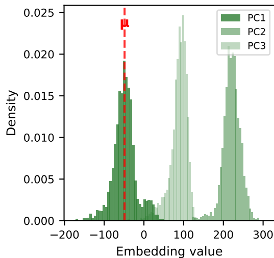
Pixel distribution
