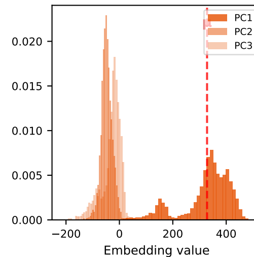
Pixel distribution
