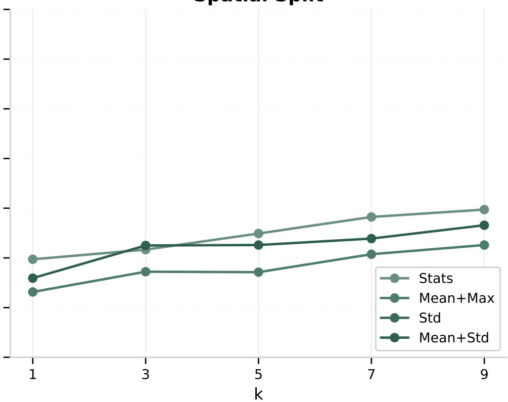
Spatial Split
