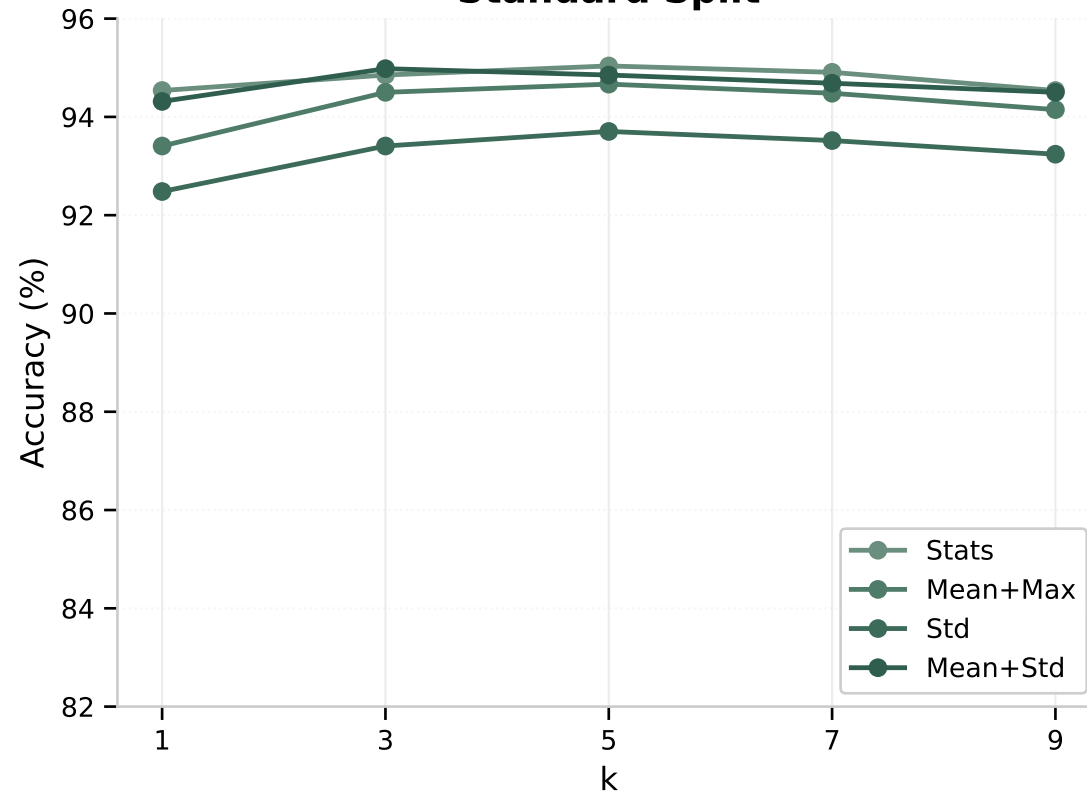
Standard Split
