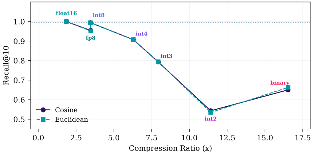
kNN Recall@10: Cosine and Euclidean
