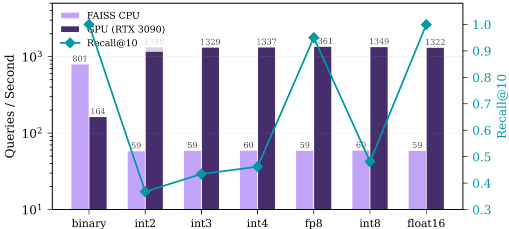
Search Throughput vs. Recall (1M corpus, 1K queries, k=10)
