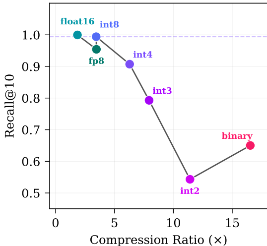
kNN Recall@10 (Cosine)
