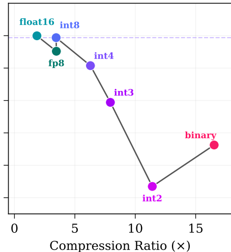
kNN Recall@10 (Euclidean)
