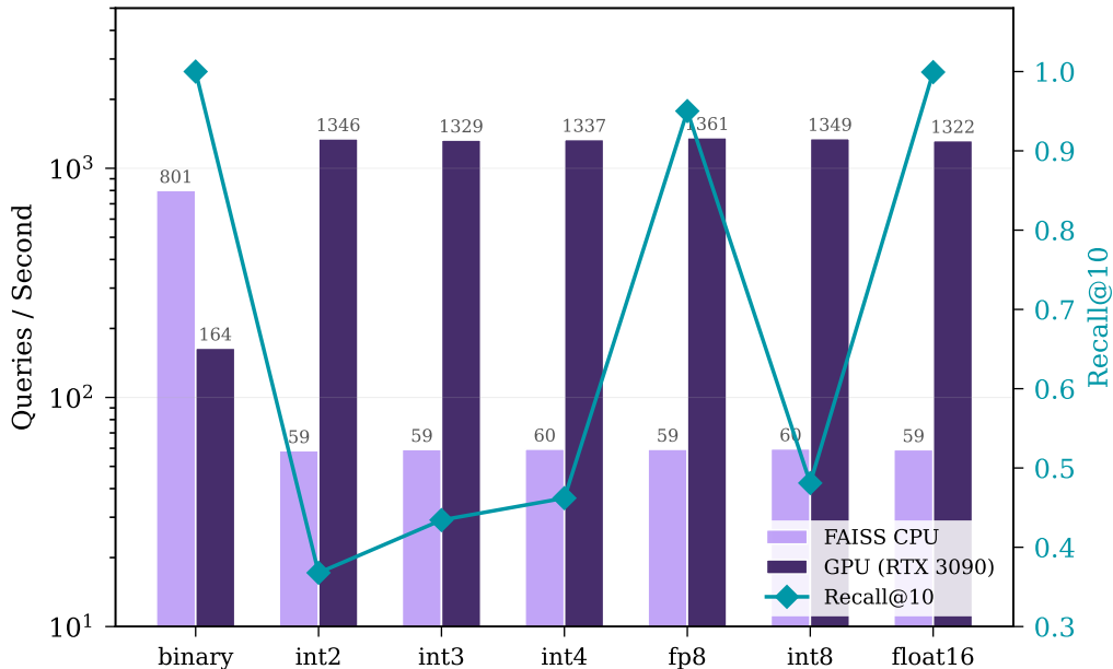
Search Throughput vs. Recall (1M corpus, 1K queries, k=10)
