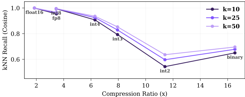
Neighborhood Preservation Across k
