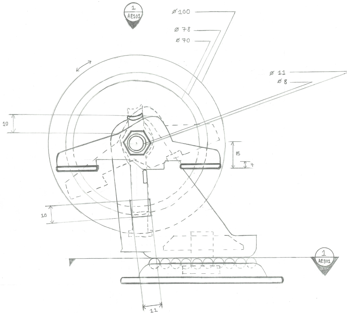
1 FRONT ELEVATION VIEW 1:1
