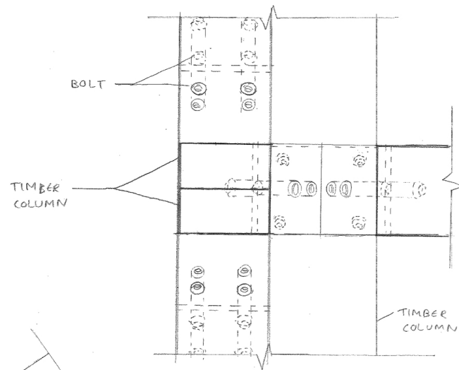
2 SIDE ELEVATION 1:5
