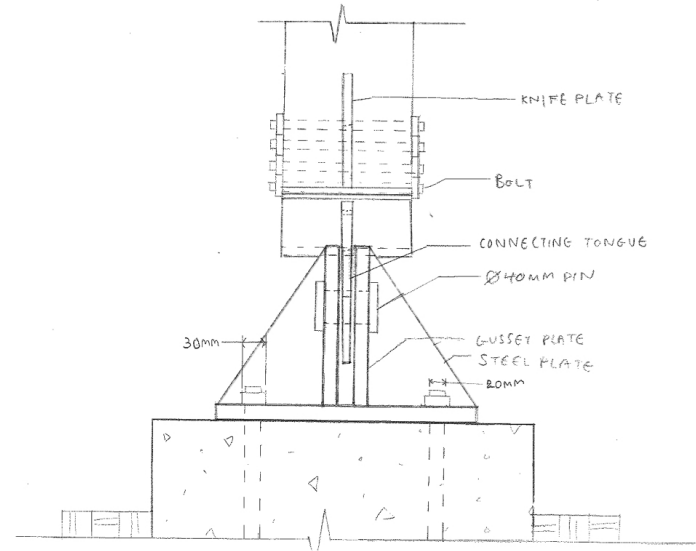
① SIDE ELEVATION 1:5
