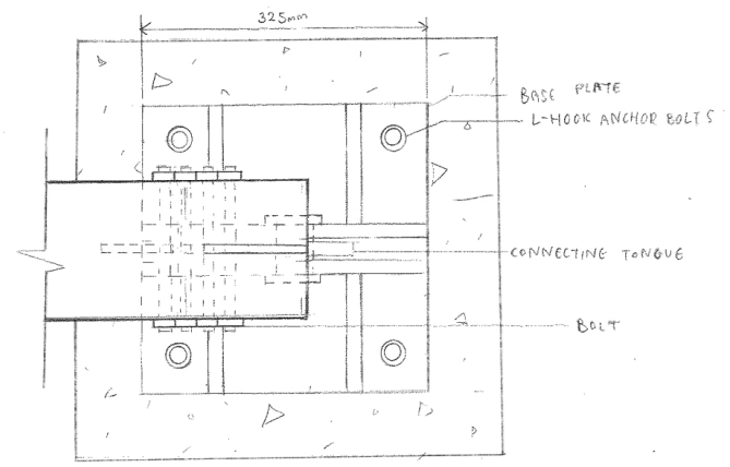
① PLAN VIEW 1:5
