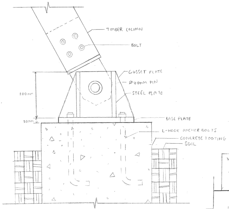
① FRONT ELEVATION 1:5
