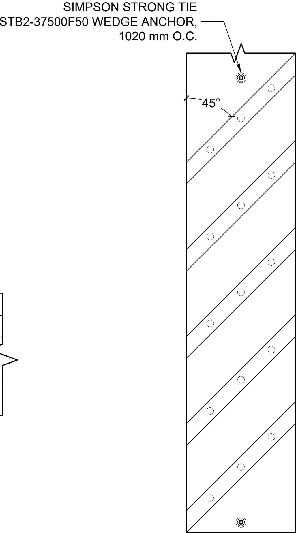
2 LOUVER PLAN VIEW 1:5
