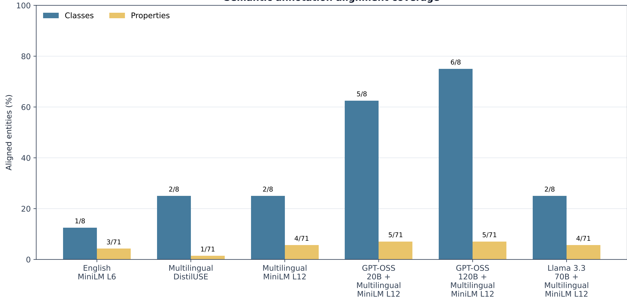
Semantic annotation alignment coverage
