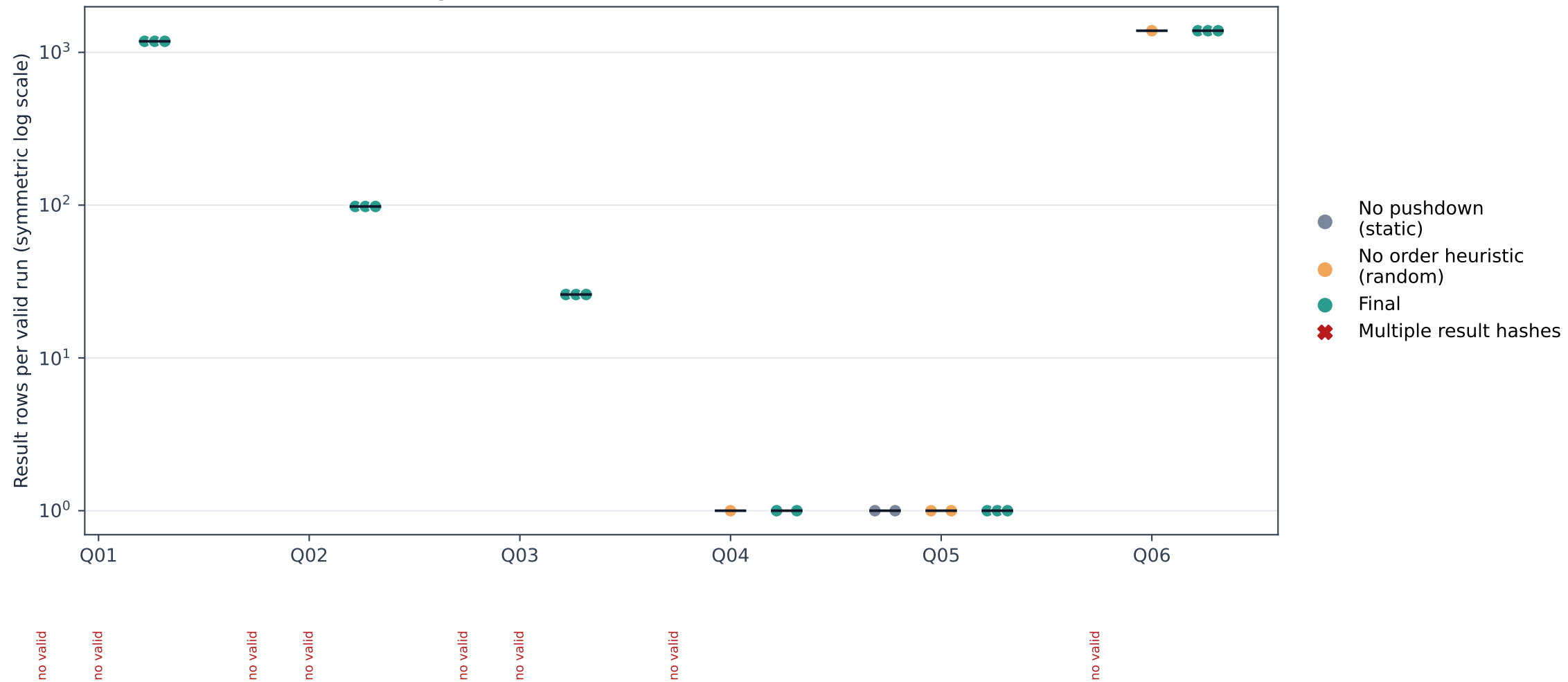
VKG result cardinality and consistency Points represent valid runs; horizontal lines show means
