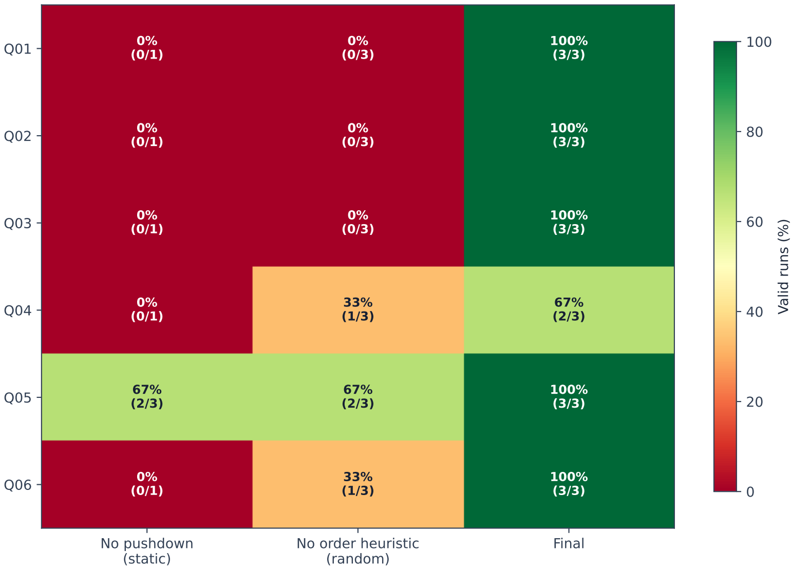
VKG valid execution rate
