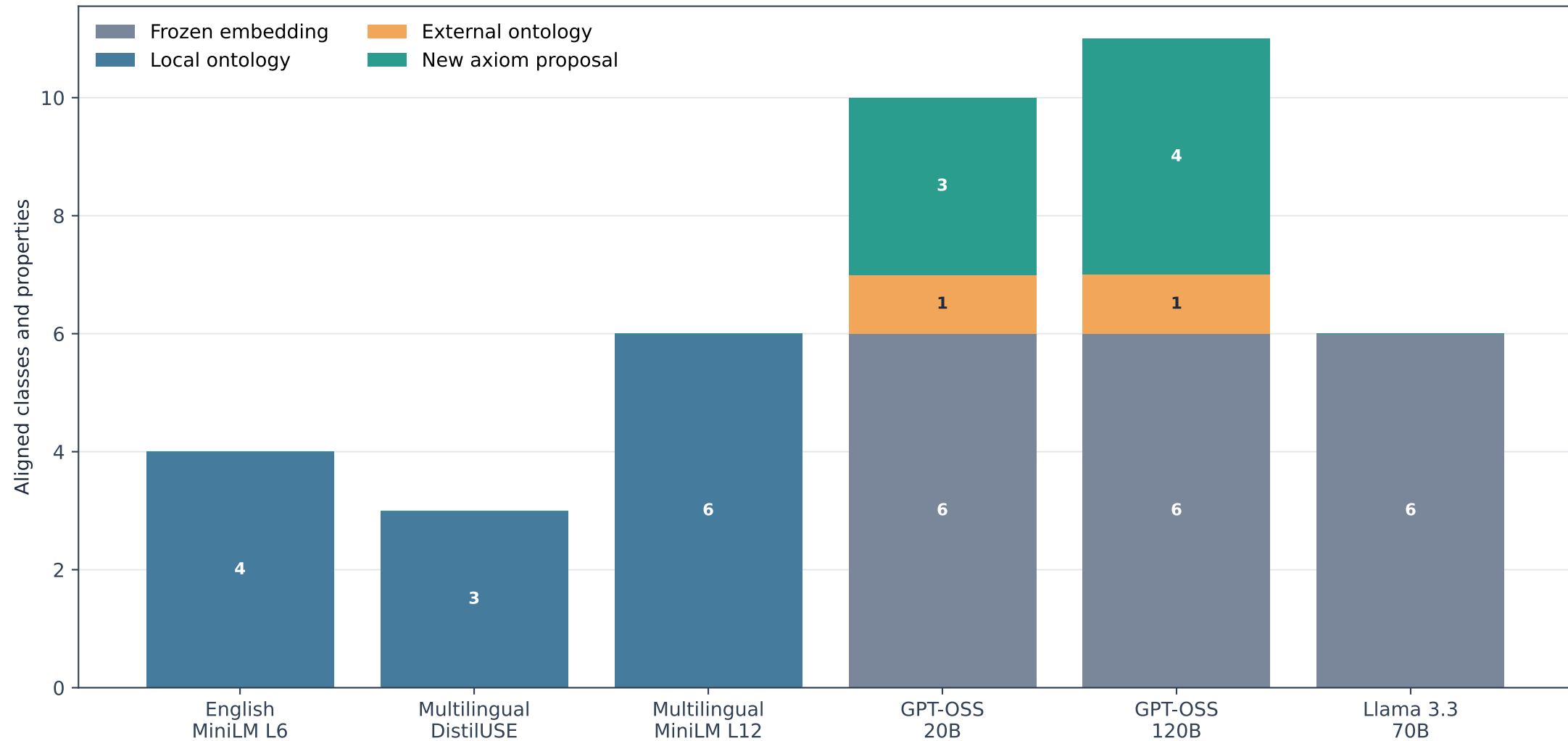
Sources of accepted semantic alignments
