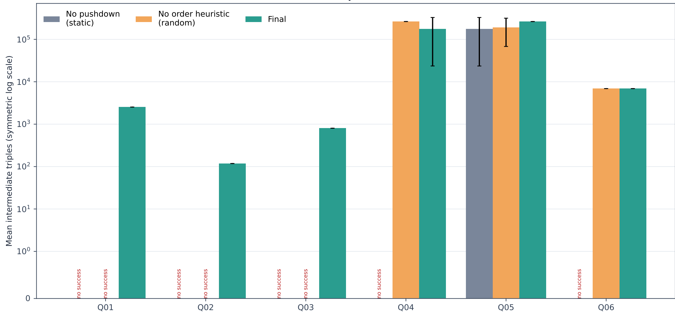
VKG intermediate triples for successful runs
