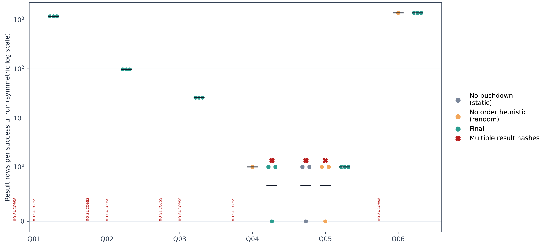
VKG result cardinality and consistency Points represent successful runs; horizontal lines show means
