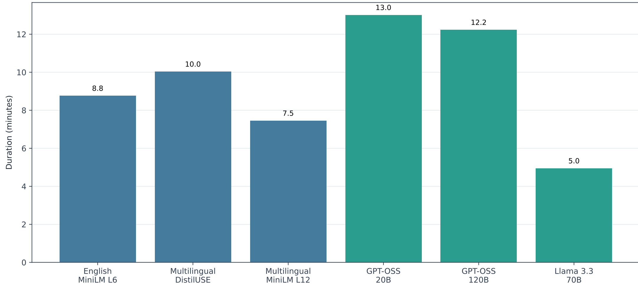
Semantic annotation execution time
