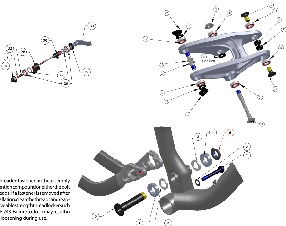
Parts for 2013-14 Fuel EX 5/ 6/ 7 Assembly
