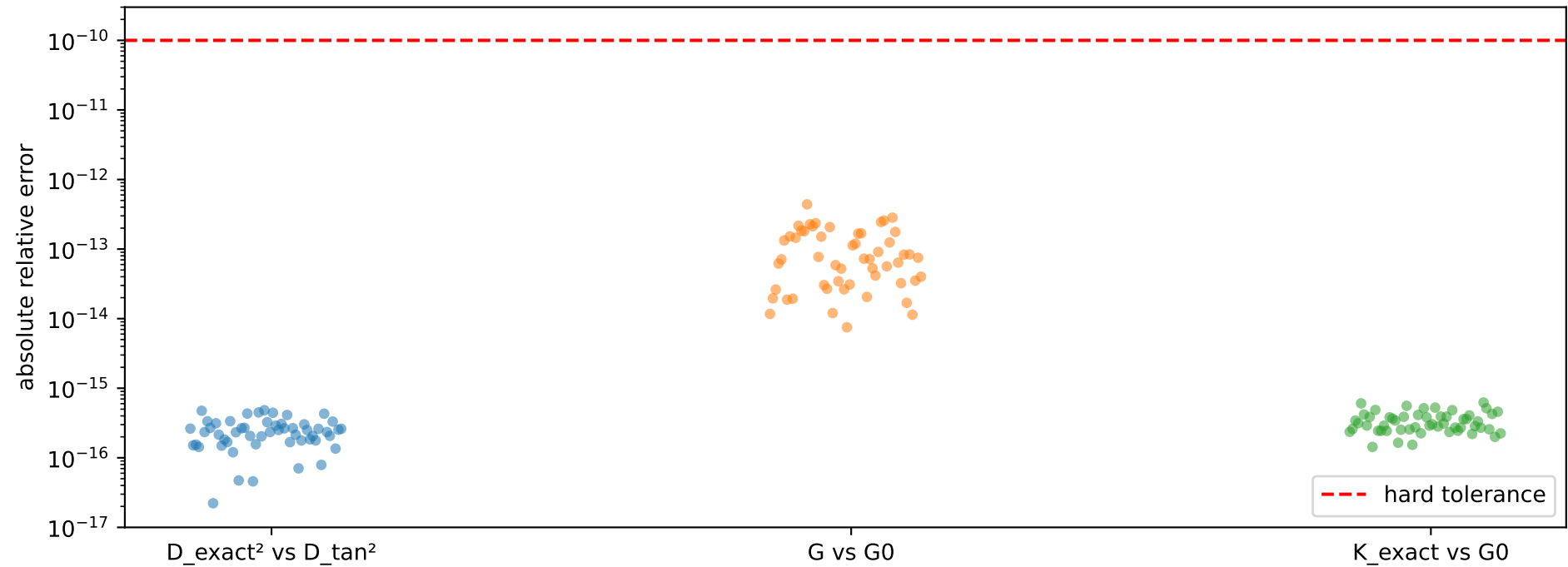
LE algebraic controls at numerical zero
