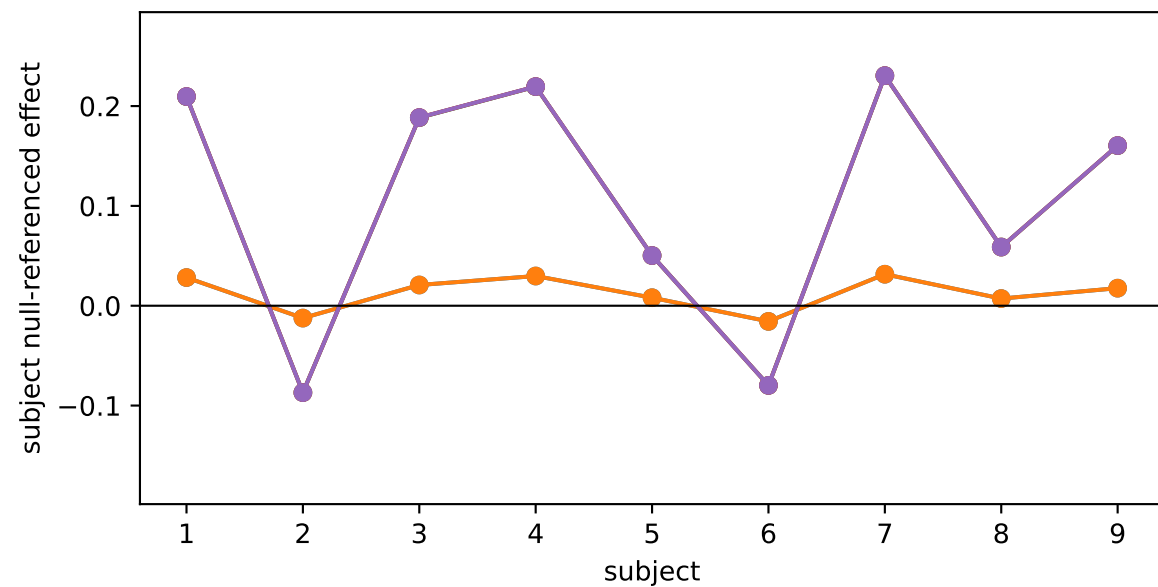
1test · AIRM
