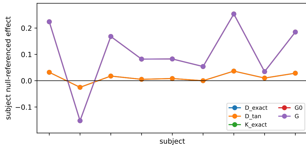
1test · AIRM
