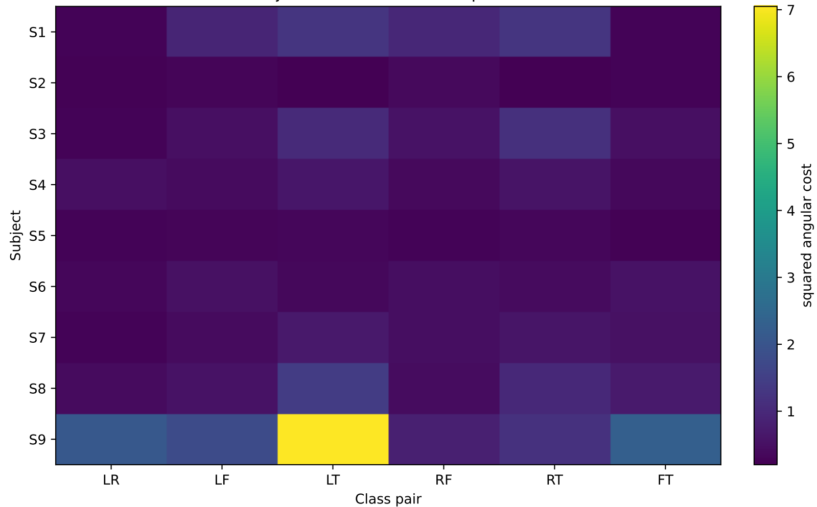
Subject-fixed class-relation profiles
