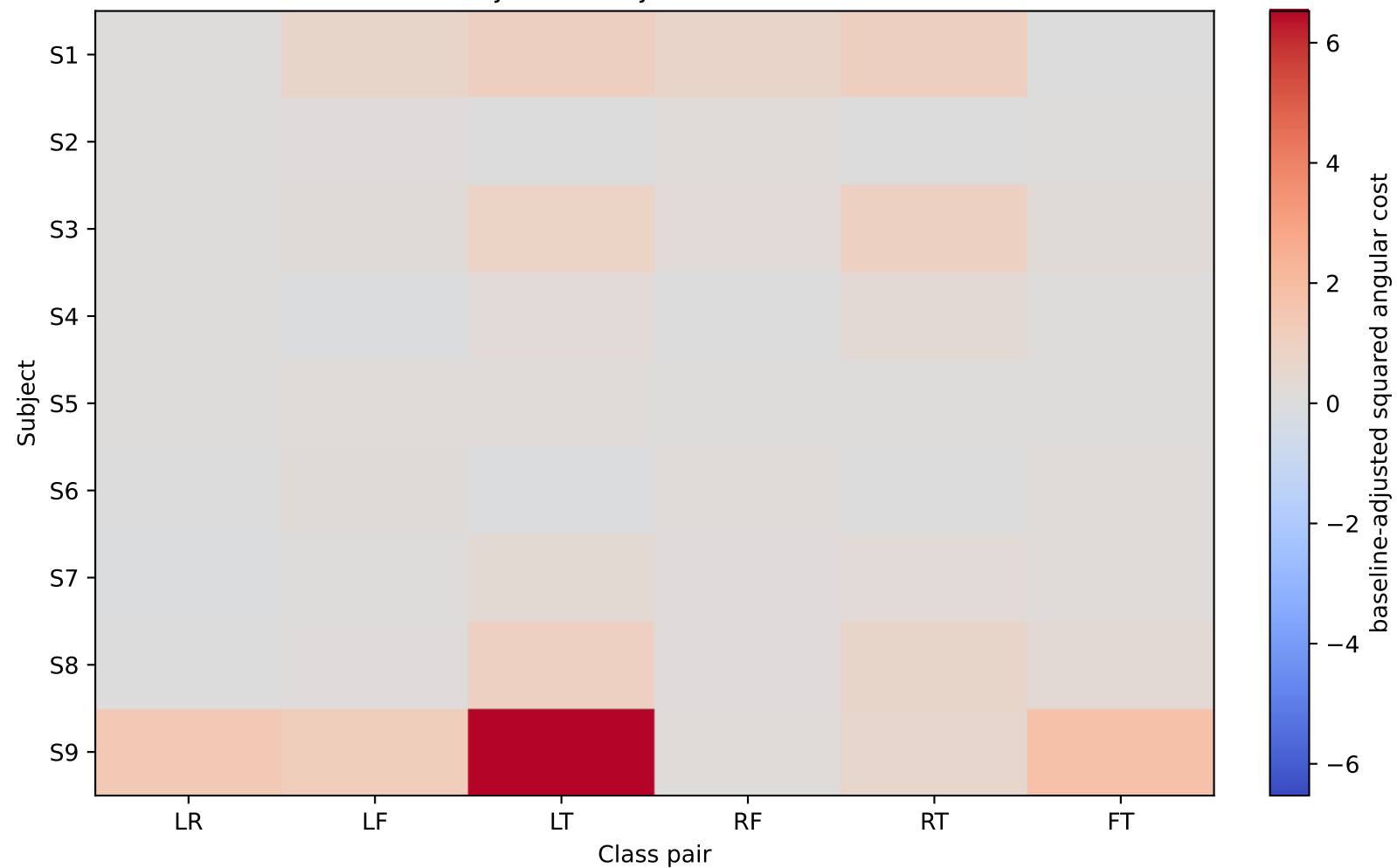
Baseline-adjusted subject-fixed class relations
