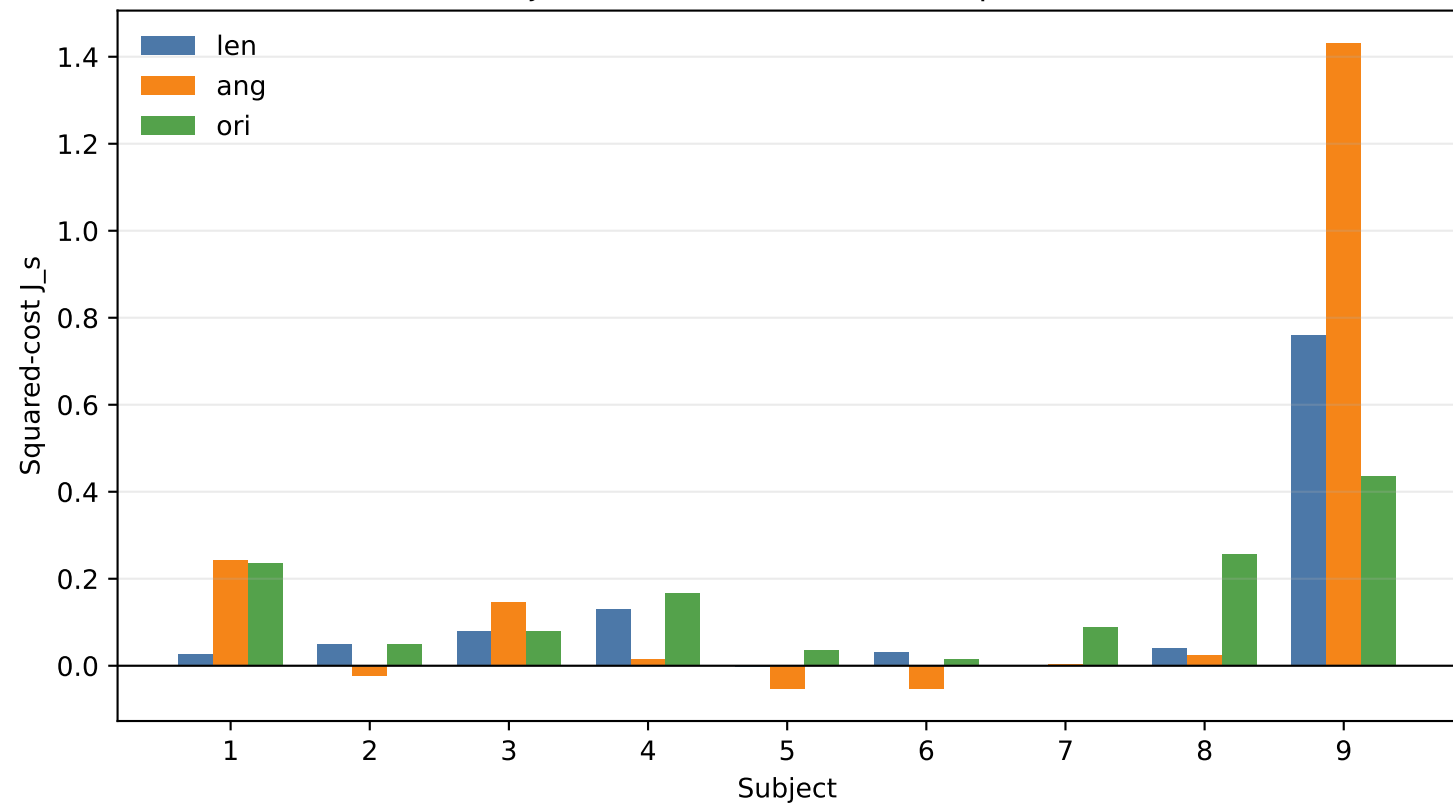
Subject-level interaction decomposition
