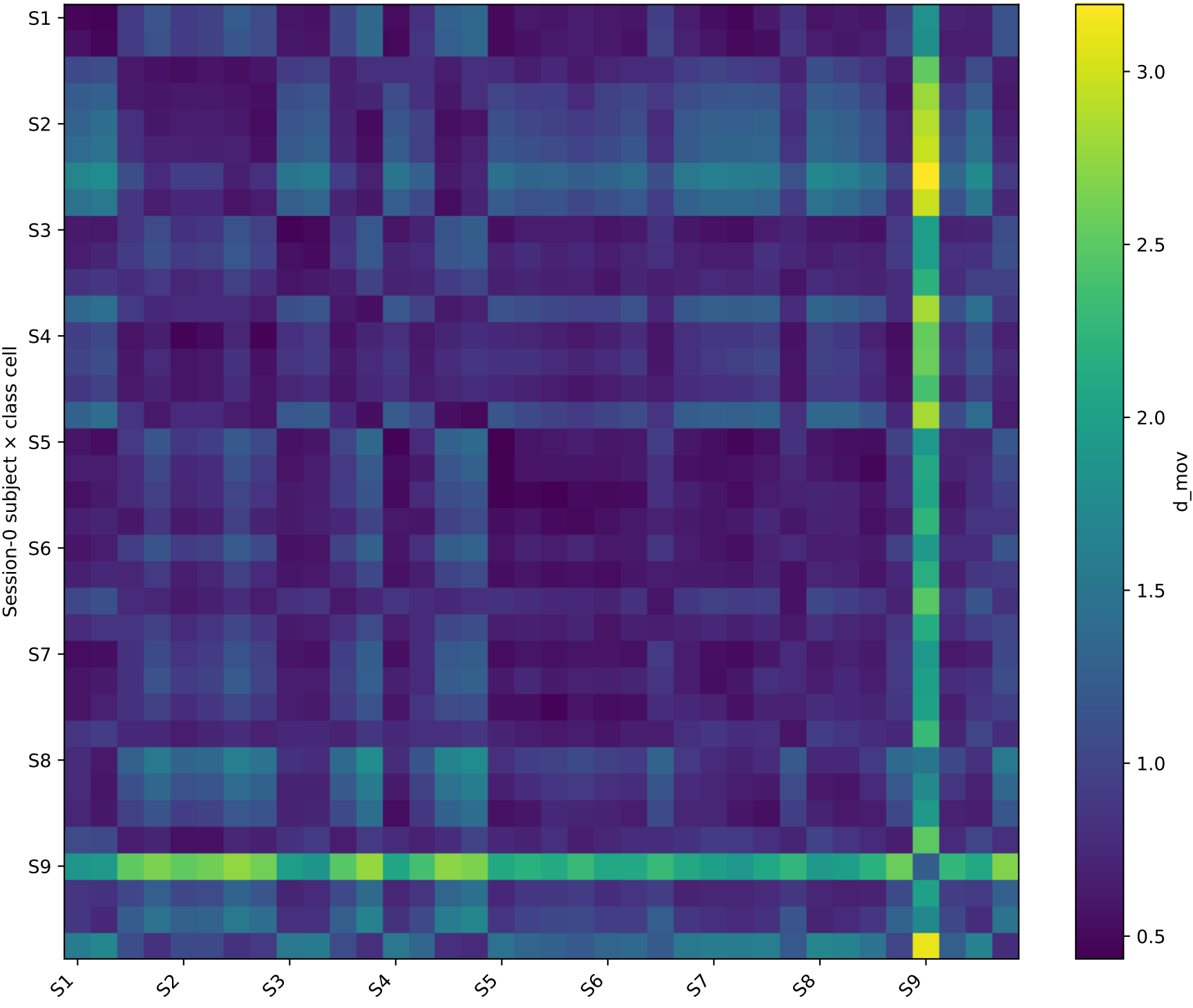
36×36 common-O quotient movement discrepancy
