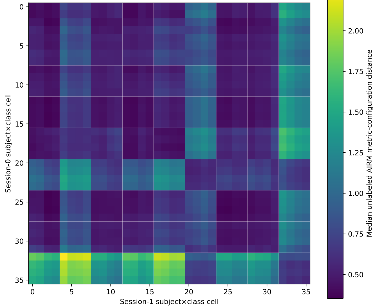
RAW directional cross-session cell distance M01
