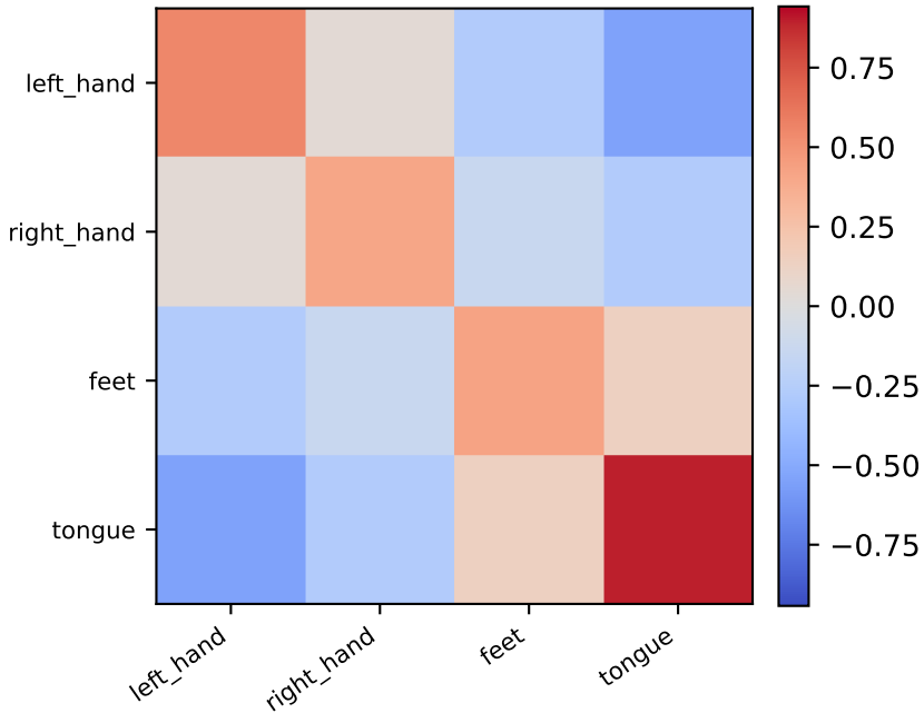
confirmatory
