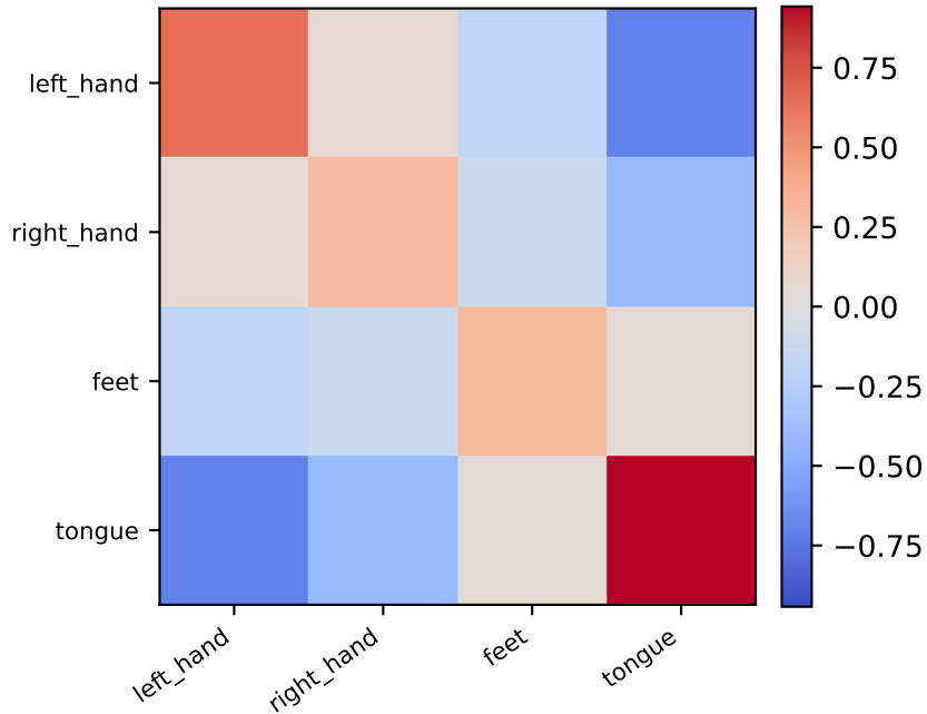
discovery
