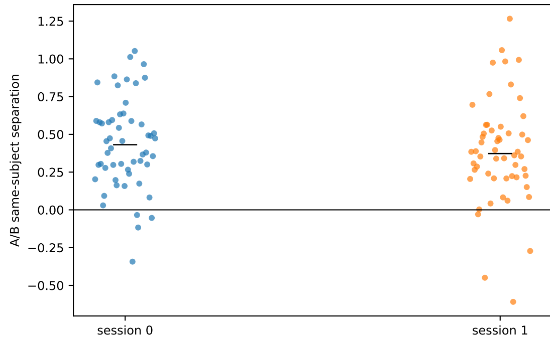
Outer-fold-safe measurement reliability
