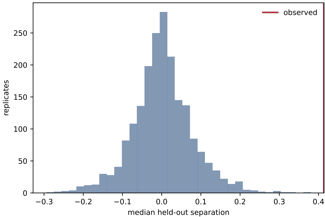
Equal-rank random subspace
