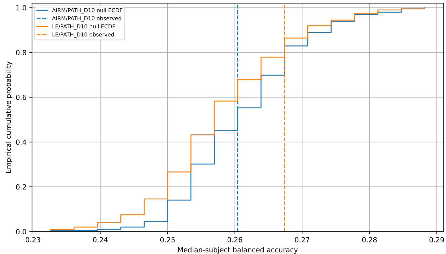
Order-shuffle falsification
