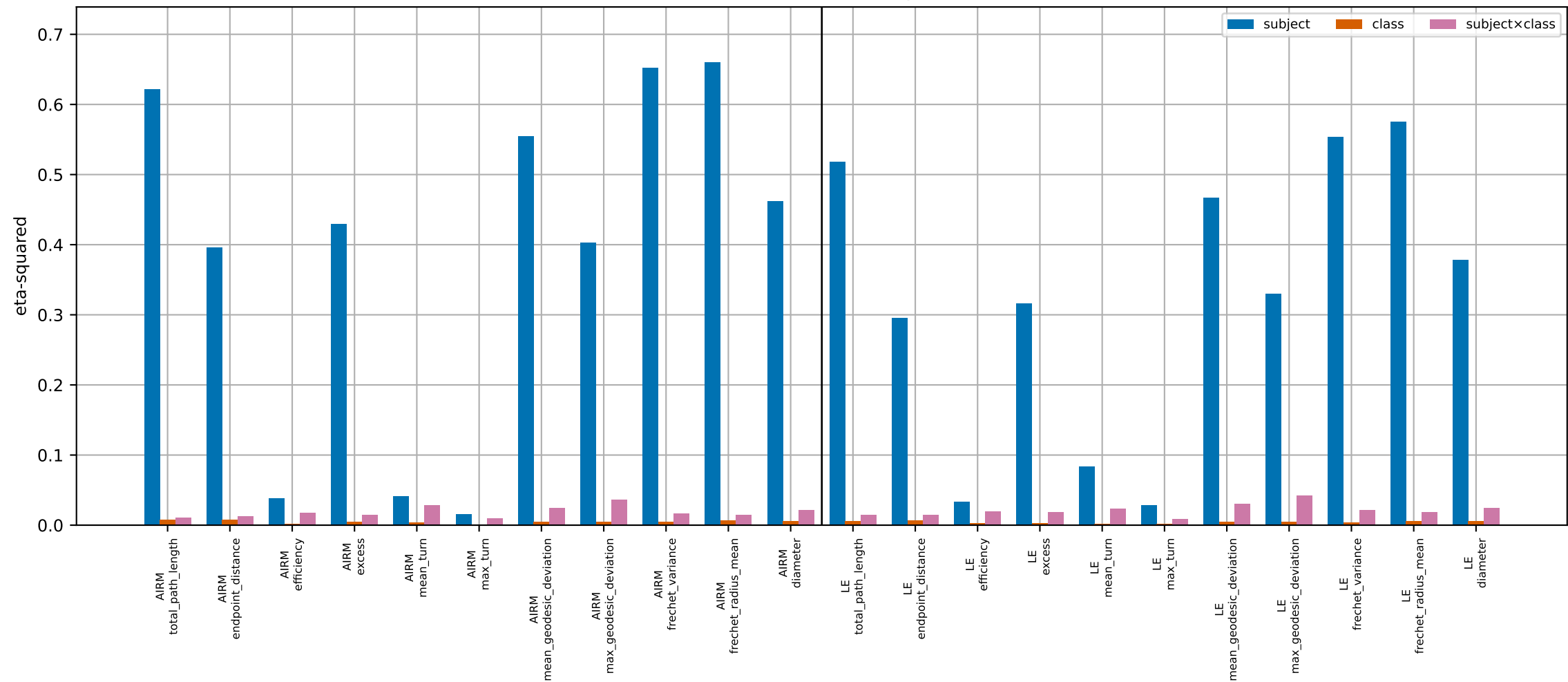
Balanced scalar variance anatomy (all 11 scalars)
