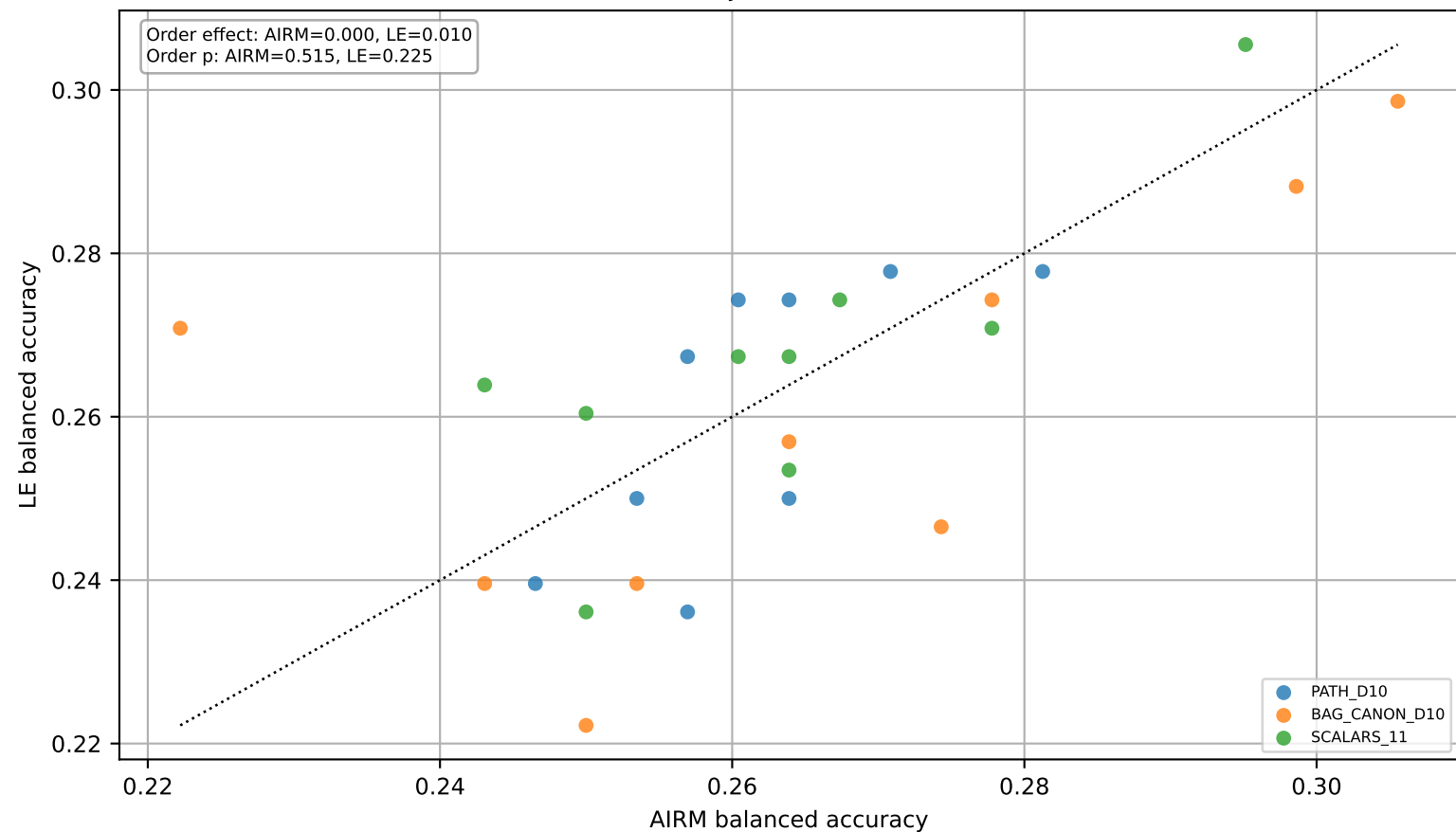
AIRM vs LE subject-wise class LOSO BA
