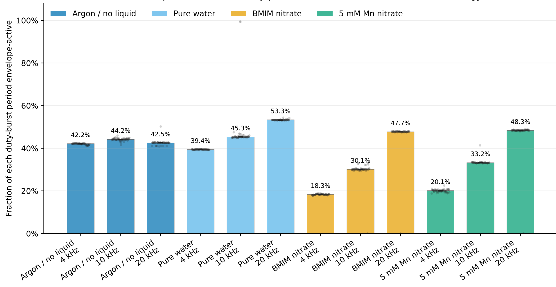
Duty-on fraction audit Same carrier-envelope threshold and duty-period windows used for lobe and Q-V energy extraction
