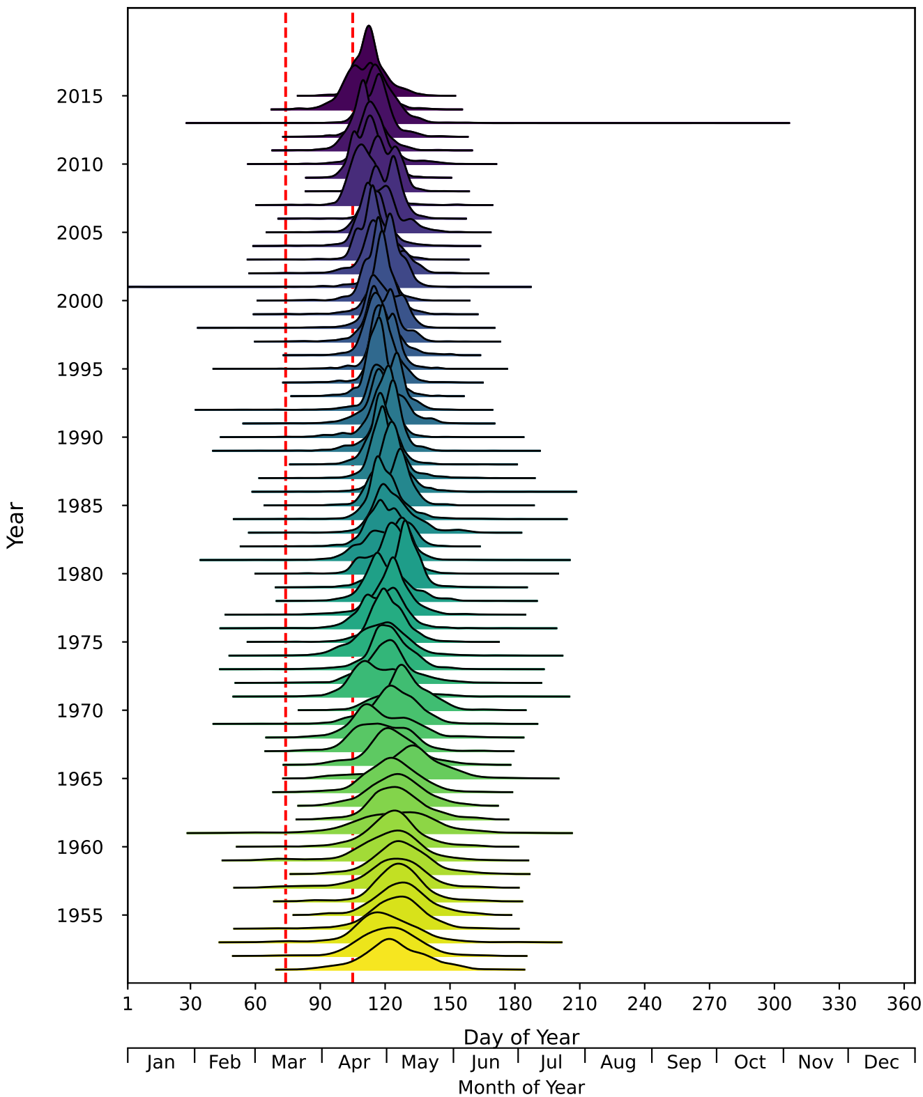
Distribution of Historical Sowing Dates by Year
